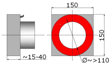
Large Area Ring Light
