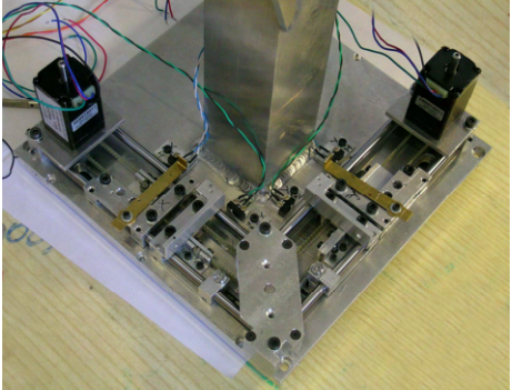
High precision aperture for neutron imaging
