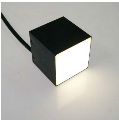
LED SPOT Backlight, 40x40mm
